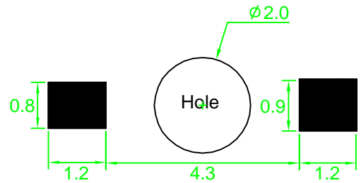
Recommended Soldering Pad Dimensions
