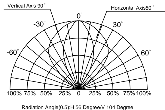
Fig.6 Directivity Radiation
