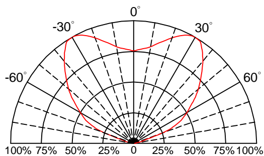
Fig.6 Directivity Radiation
