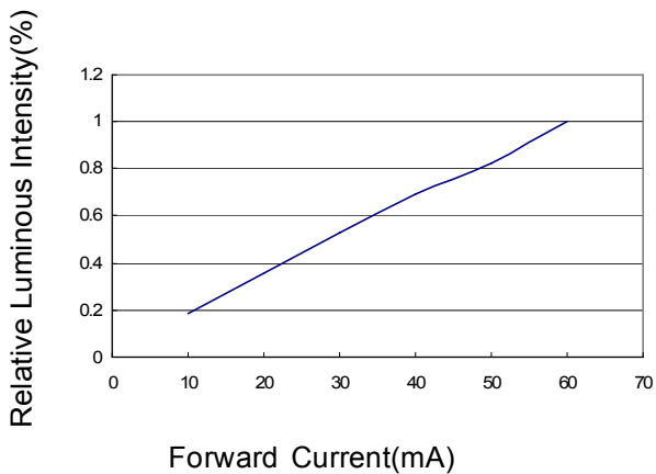
Fig.2 Forward current vs. Luminous Intensity
