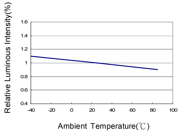
Fig.4 Luminous Intensity vs. Temperature
