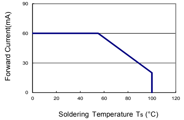
Fig.3 Max. Driving Forward Current VS. Soldering Temperature
