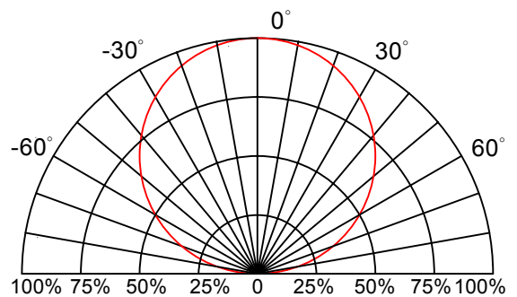
Fig.6 Directive Radiation
