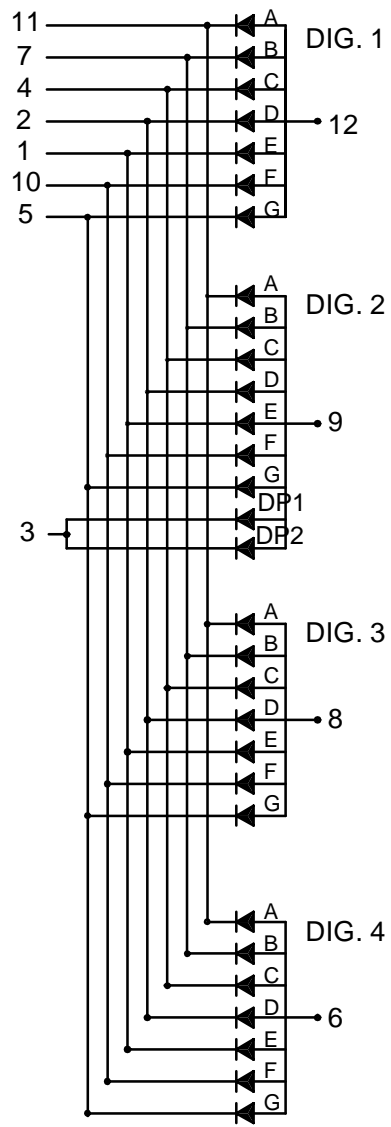
LFD2125-XX
