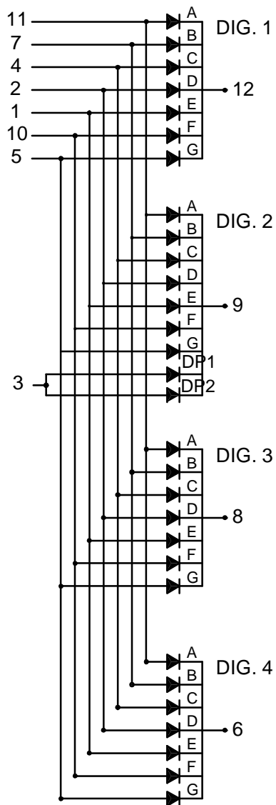
LFD2115-XX
