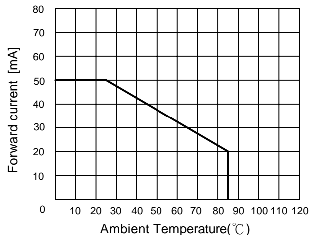
Fig.6 Operation Temperature Range
