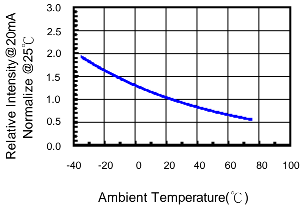
Fig.6 Operation Temperature Range
