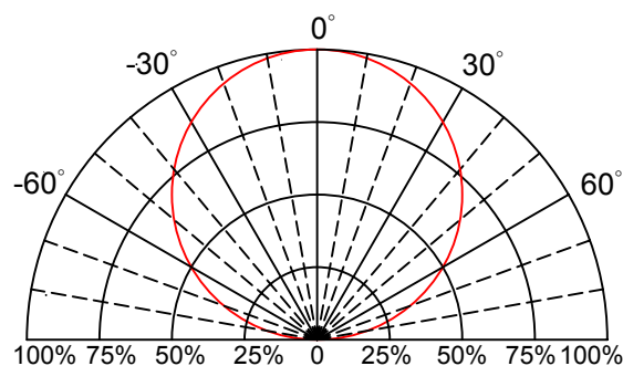
Fig.6 Directive Radiation
