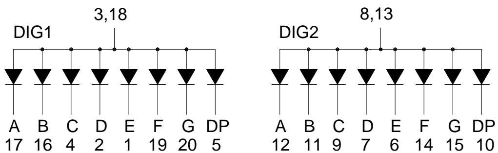
LSDD206A-XX(Common Anode)
