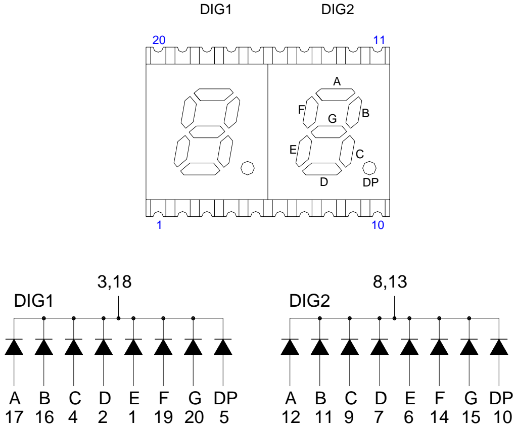
LSDD205A-XX(Common Cathode)
