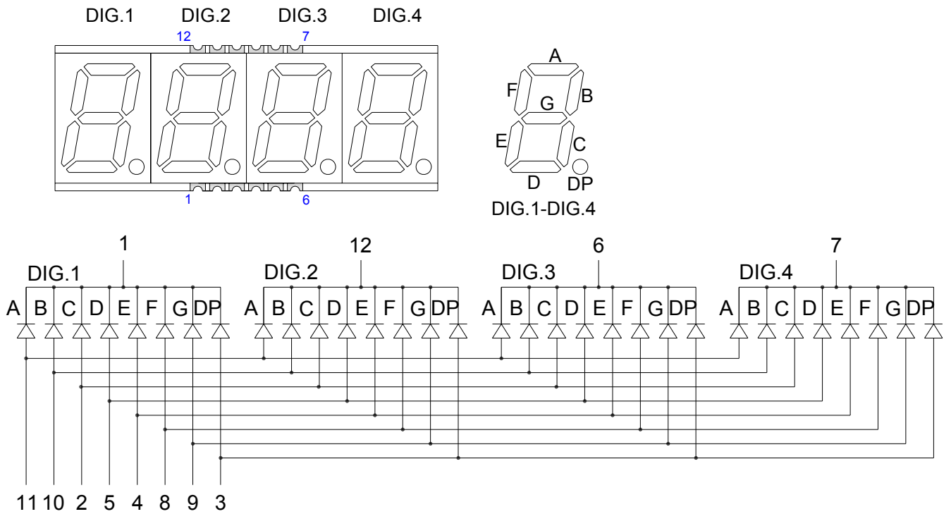
LSFD5156F-XX (Common Cathode)
