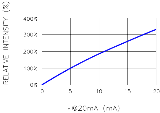
Fig.1 RELATIVE INTENSITY VS. FORWARD CURRENT
