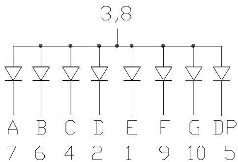
LSSD306A-XX (Common Anode)
