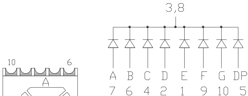
LSSD305A-XX (Common Cathode)
