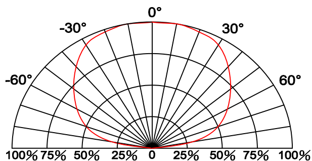
Fig.6 Directive Radiation
