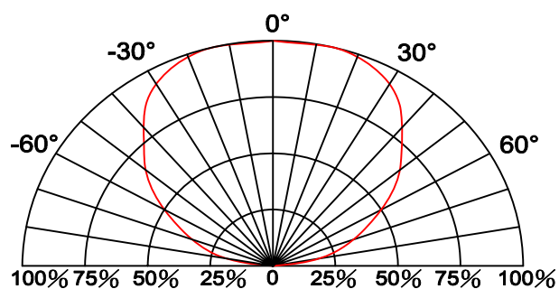
Fig.6 Directive Radiation
