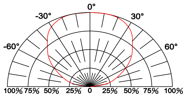
Fig.6 Directive Radiation
