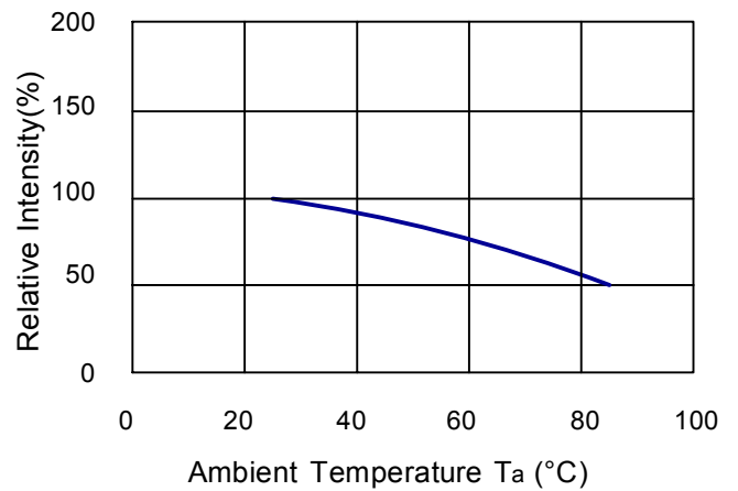
Fig.4 Relative Intensity VS. Ambient Temperature
