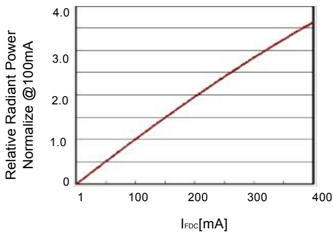
Fig.3 Relative Radiant Power vs. Forward DC Current
