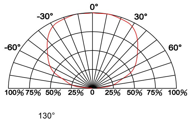
Fig.6 Directive Radiation
