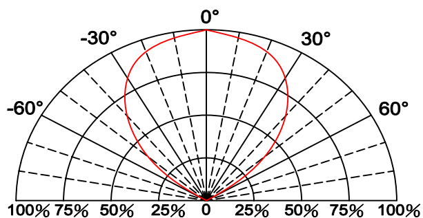
Fig.5 Directive Radiation
