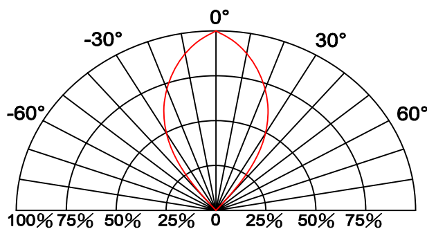
Fig.5 Directive Radiation
